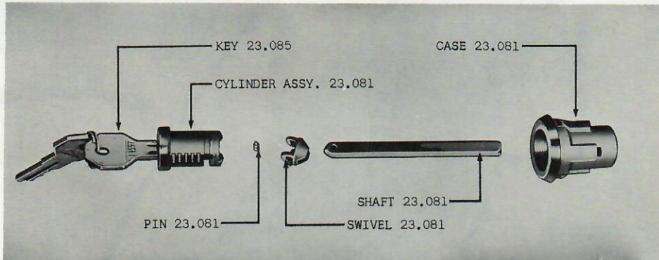
GROUP 23 - FIG. 12 - DOOR LOCK CYLINDER AND KEYS 01-10-20-80
