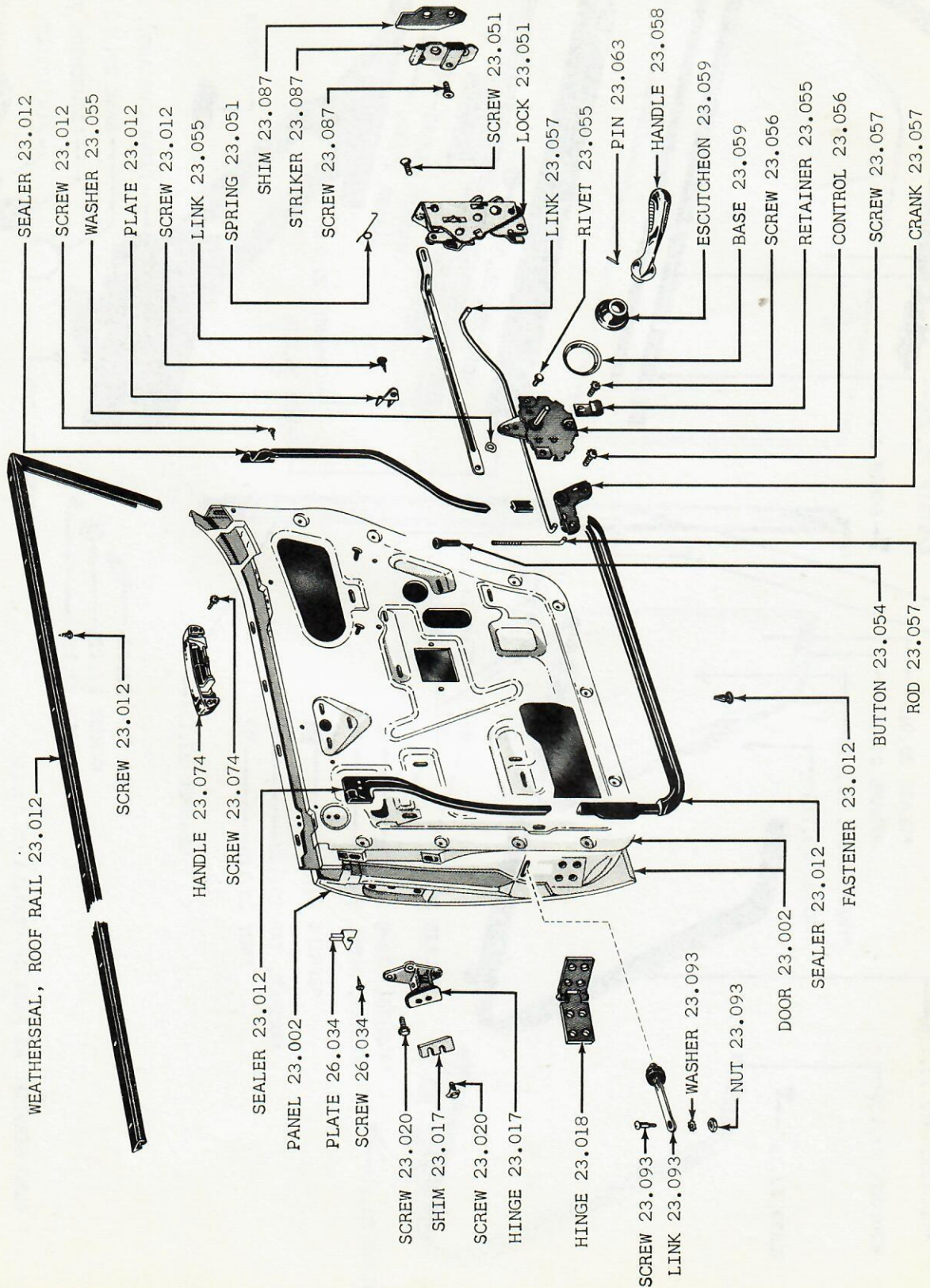
GROUP 23 - FIG. 5 - REAR DOOR, HARDWARE AND SEALERS 19-23-29-83-89
