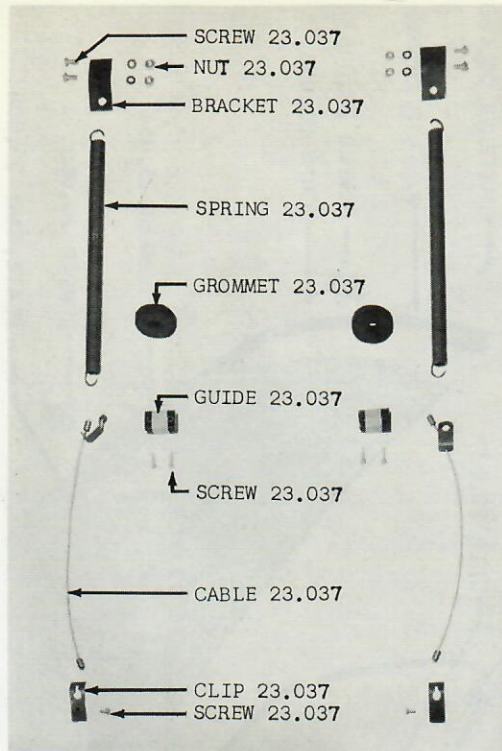
GROUP 23 - FIG. 11 - TAILGATE COUNTERBALANCE ASSEMBLY 18-28-83-88
